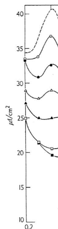
Fig. 1. Differential ce of salmon sperm DNA --- no DNA; ▲ — C_b = 0.16 r
