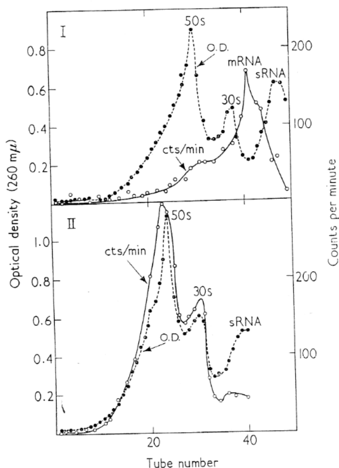
FIG. 8. Incorporation and turnover of uracil in messenger RNA. E. coli growing exponentially in broth were incubated for 5 sec with [ ^{14}C ]-uracil. The bacteria were centrifuged, washed and resuspended in the original volume of the same medium containing 100-fold excess of [ ^{14}C ]-uracil. Half the bacteria were then harvested and frozen (I) and the remainder were incubated for 15 min at 37°C (II) prior to harvesting and freezing. The frozen samples were ground with alumina and extracted with tris buffer (2-amino-2 hydroxymethylpropane-1:3-diol) containing 10^{-4}M -Mg, treated with DNase and applied to a sucrose gradient. After 3 hr, sequential samples were taken for determination of radioactivity and absorption at 260 mμ. It may be seen (part I) that after 5 sec, M-RNA is the only labelled fraction, and that subsequently (part II) uracil incorporated into M-RNA is entirely renewed. (From Gros et al. , 1961.)
